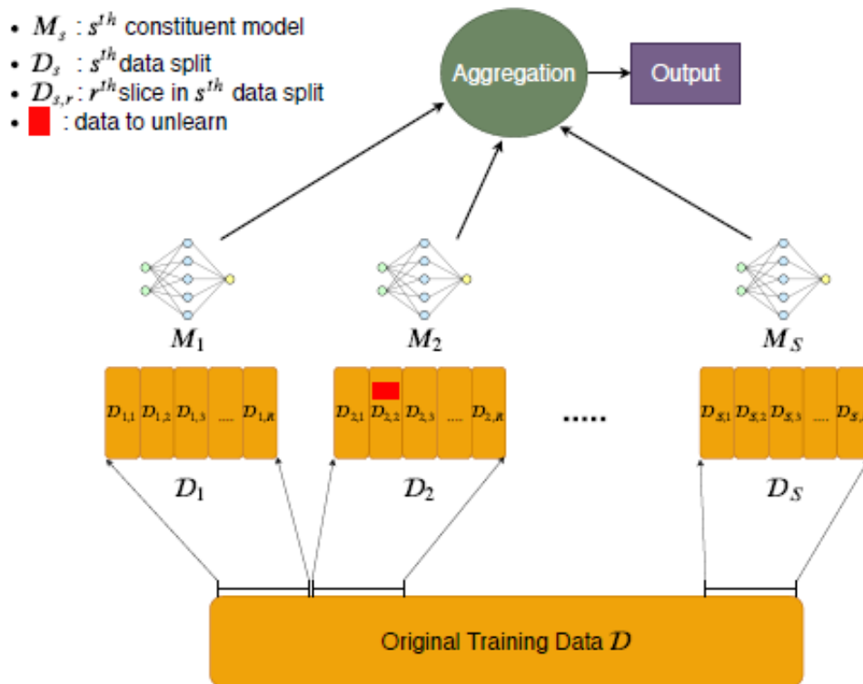
Figure 10 : SISA Training Architecture [15]
